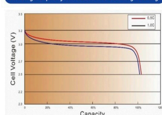
Discharge Capacity In Relation To Discharge Voltage
