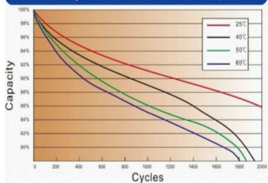
Temperature Effect In Relation To Battery Capacity
