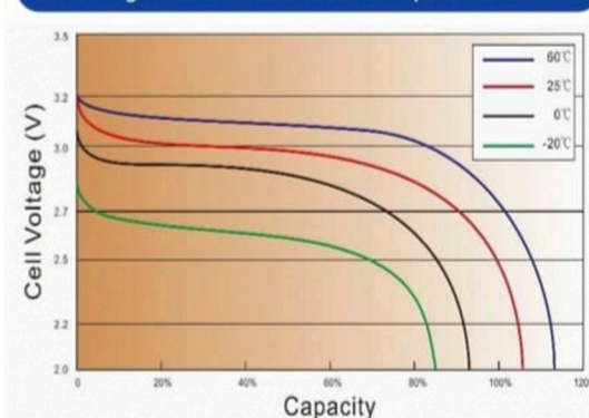
Discharge Curve At Different Temperature ( 1C )
