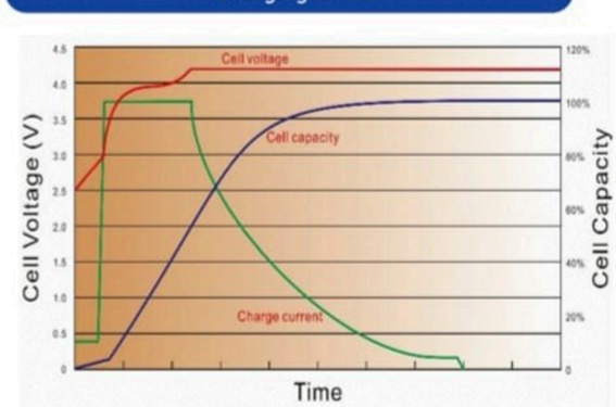
Charging Curve
